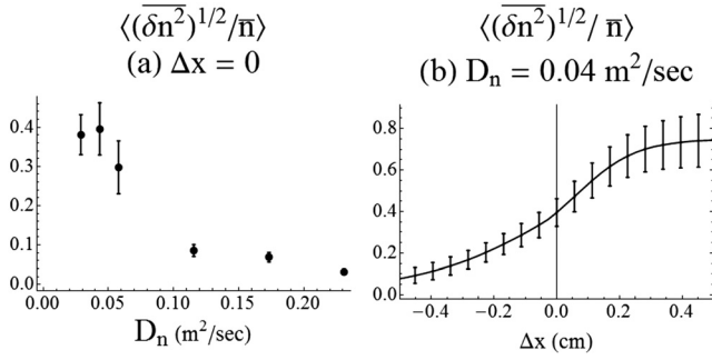
FIG. 2. Relative density fluctuation: the time-averaged r.m.s. density fluctuation, with respect to y , divided by the y -averaged density, in the simulations, (a) measured at the separatrix, versus the density diffusion coefficient D_n , and (b) versus radius ( \Delta x ) for D_n = 0.04 \text{ m}^2/\text{s} . The over-bar denotes the y -average; the angular brackets denote the time-average; error bars are standard deviations with respect to time, and the sample was restricted to the steady state in each case.
