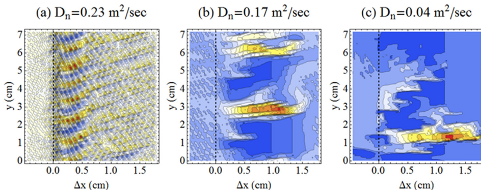
FIG. 3. Snapshots of the instantaneous density fluctuation divided by the y -averaged density, (n - \bar{n})/\bar{n} from the simulations for (a) D_n = 0.23 \text{ m}^2/\text{s} , in the weak-turbulence, possibly sub-threshold, regime, (b) D_n = 0.17 \text{ m}^2/\text{s} , over threshold, where streamers are observed, and (c) D_n = 0.04 \text{ m}^2/\text{s} , in the strong turbulence regime where isolated blobs are observed in the SOL.
