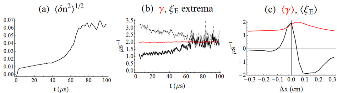
FIG. 6. For the simulation with D_n = 0.17 \text{ m}^2/\text{s} , starting from small-amplitude noise: (a) the density fluctuation (normalized to the separatrix value) versus time; (b) the maximum value of the interchange growth rate, \gamma = \sqrt{-\beta \cdot \partial_x (\bar{p}_e + \bar{p}_i) / \bar{n}} (red), the maximum value of the shearing rate of the mean E \times B flow, \zeta_E = \partial_x \bar{v}_E (black), and the magnitude of the minimum value of \zeta_E (black dotted) versus time; (c) the time-average of the growth rate and of the shearing rate, over the last 20 \mu\text{s} in (b), versus \Delta x . In (a), the angular brackets denote the spatial average over the simulation box. In (b), the extrema of \zeta_E and the maximum of \gamma are located within |\Delta x| < 3 \text{ mm} , but are not coincident, as seen in (c).
