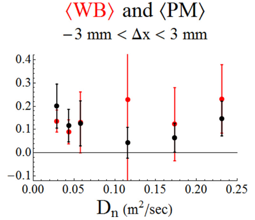
FIG. 9. Wave-breaking (WB, red) and profile modification (PM, black) parameters, Eqs. (7) and (8), respectively, averaged over the radial interval |\Delta x| < 3 \text{ mm} versus the density diffusion coefficient D_n . Error bars are standard deviations with respect to the average.
