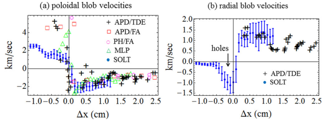
FIG. 5. Poloidal (a) and radial (b) components of the correlation velocity for the strong-blobby simulation ( D_n = 0.04 \text{ m}^2/\text{s} ) are plotted (dots with error bars) versus radius and compared with different measures of the corresponding velocity components of fluctuations in the discharge. In (a) and (b), (+) denotes time-delay estimation (TDE) analysis of GPI data captured by the avalanche photo-diode (APD) array. In (a), ( \square ) denotes Fourier analysis (FA) of GPI data captured by the APD array, (O) denotes FA of GPI data captured by the Phantom camera (PH), and ( \Delta ) denotes 2-point phase-delay analysis of fluctuations measured by the MLP.
