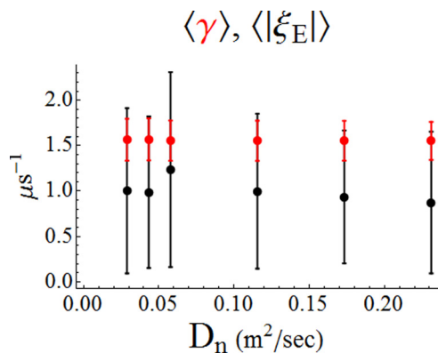
FIG. 7. Time- and x -averages of the interchange growth rate, \langle \gamma \rangle (red), and of the E \times B flow shearing rate, \langle \zeta_E \rangle (black), versus the density diffusion coefficient D_n . The x -average is restricted to a \pm 3 mm neighborhood of the separatrix, and the time-average is taken over times long compared to the fluctuation time scale in equilibrium in each case. The error bars are standard deviations with respect to the x -average.
