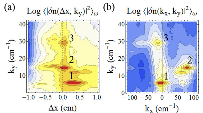
FIG. 8. Energy spectra of the density fluctuations from the weak-turbulence simulation, D_n = 0.23 m 2 /s. The frequency-averaged spectrum is plotted as a function of (\Delta x, k_y) in (a) and as a function of (k_x, k_y) in (b). Three prominent maxima (or waves), labeled, are discussed in the text. Wave (2) corresponds to the separatrix-spanning interchange mode in Fig. 4(a) and drives the turbulence in the near-SOL.
