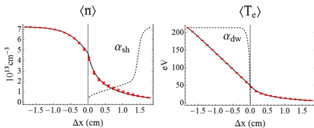
FIG. 1. Time-averaged density and temperature profiles from a simulation ( D_n = 0.04 m 2 /s) plotted as discrete points (red). The height of the point symbol is the standard deviation with respect to time, seen to be negligible on the scale of the plot. Also plotted are the reference density and electron temperature profiles (solid) for the discharge, and the sheath ( \alpha_{sh} ) and drift wave ( \alpha_{dw} ) coefficients (dashed), rescaled to fit the plot. The over-bar denotes the y -average, and the angular brackets denote the time-average.
