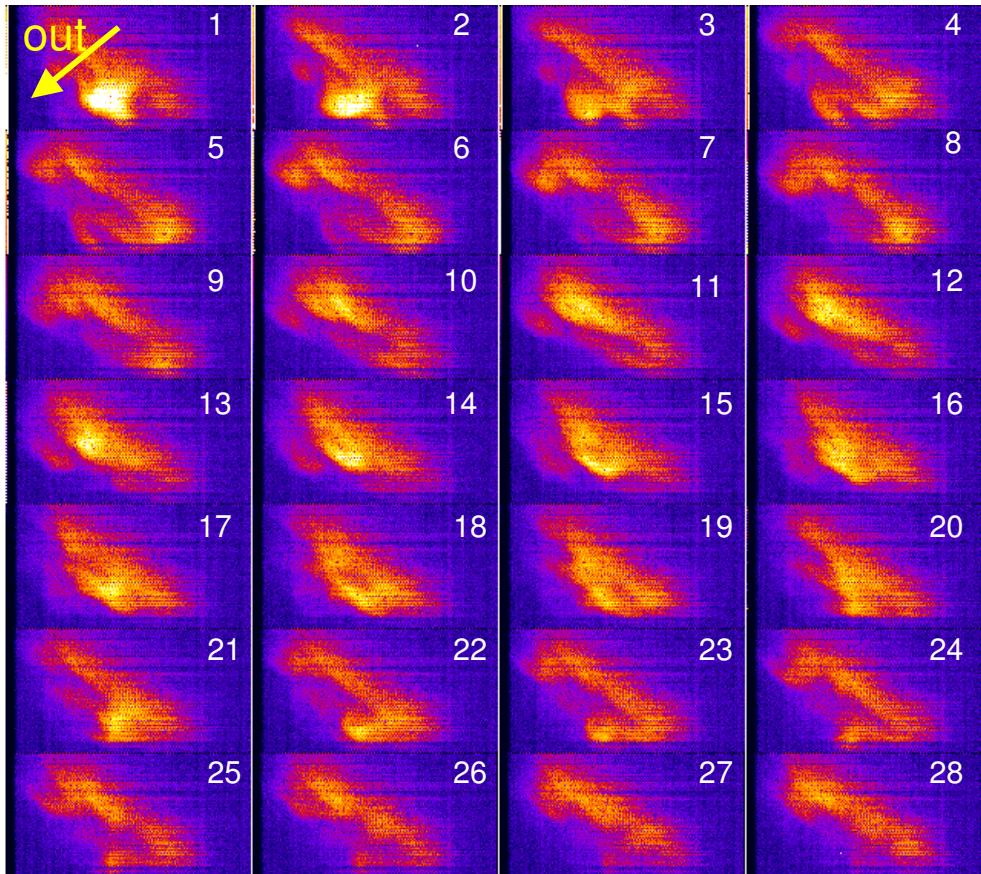
Fig. 1: Edge turbulence images from NSTX at 100,000 frames/sec showing a region \approx 30 cm \times 15 cm near the outer midplane with the outer wall toward the lower left corner.
