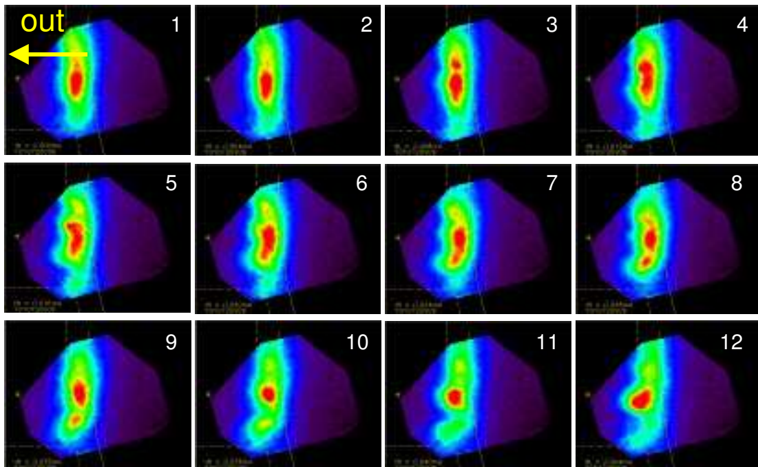
Fig. 2 – Edge turbulence images from Alcator C-Mod at 250,000 frames/sec showing a region \approx 6 cm \times 6 cm near the outer midplane with the outer wall toward the left.
