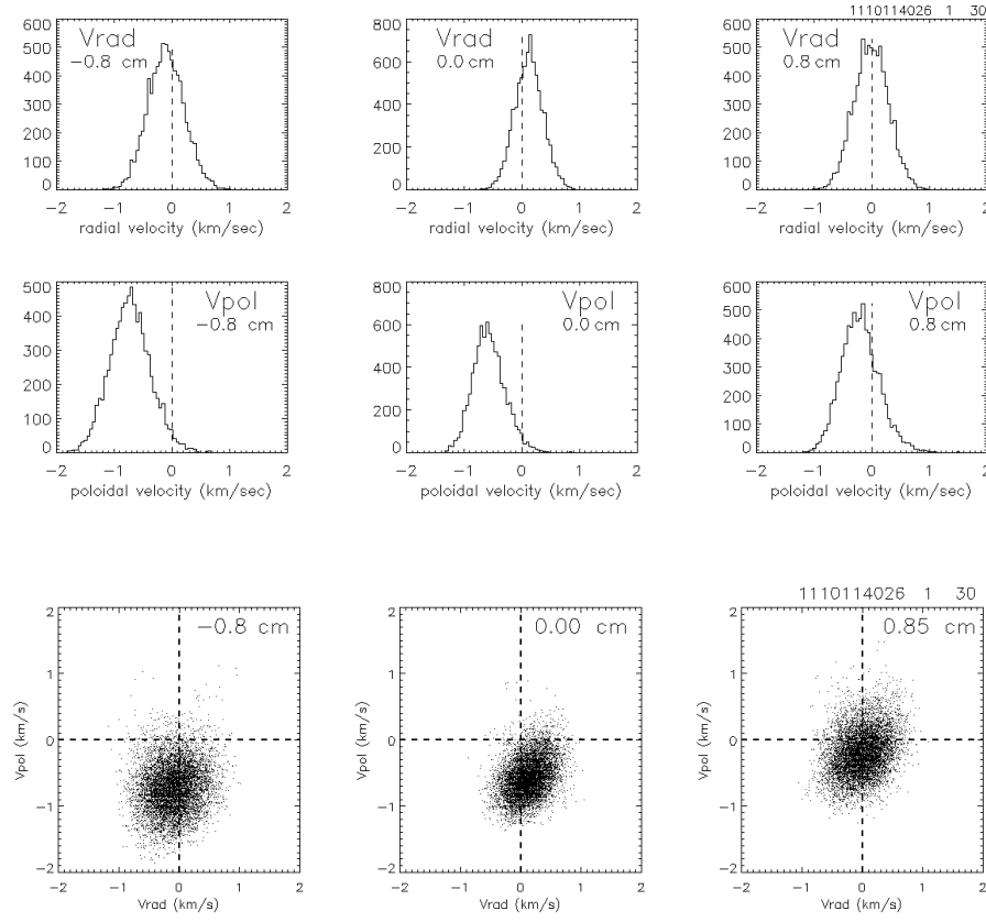
Fig. 8 - The top two panels show the probability distribution functions of V_{\text{rad}} and V_{\text{pol}} for three different radial locations in one shot (1110114026), averaged over 20 msec. The velocities have a large spread around their mean values in all cases. The bottom panel shows distributions of V_{\text{rad}} vs. V_{\text{pol}} for each time point for the cases above for the three different radial locations in 1110114026. There is a significant correlation between V_{\text{rad}} and V_{\text{pol}} at \rho = -0.8 cm and \rho = 0 cm.
