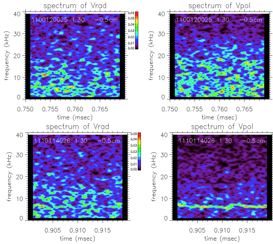
Fig. 9 – Examples of frequency spectra of V_{\text{rad}} and V_{\text{pol}} for \rho = -0.5 cm for two shots (1100120025 and 1110114026). The amplitude spectrum of V_{\text{pol}} is broadband and intermittent for shot 100120025, but has a near-coherent component at 6-7 kHz for shot 1110114026. The V_{\text{rad}} do not have a clear coherent feature in the latter case.
