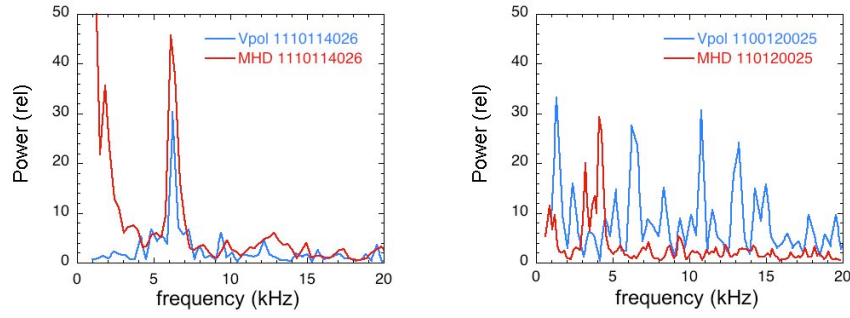
Fig. 14 – Comparison of the frequency spectra of V_{\text{pol}} at \rho = 0 cm for the two shots of Figs. 9 and 11 with the MHD spectrum from a B-dot coil at the wall, both averaged over 20 msec. There is a coincidence between the V_{\text{pol}} oscillation at 6-7 kHz and the MHD in the case at the left, but no correlation of these features in the case at the right.
