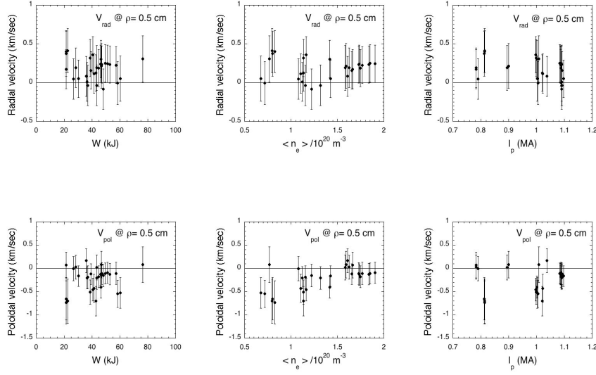
Fig. 7 – Poloidal and radial velocities at \rho=0.5 cm for the 30 shots in this database as a function of three global plasma parameters, W (stored energy), \langle n_e \rangle (line-averaged density), and I_p (plasma current). The RMS deviations from these average velocities are shown by the error bars. There is no clear variation in either the mean or RMS velocities with these parameters in this database.
