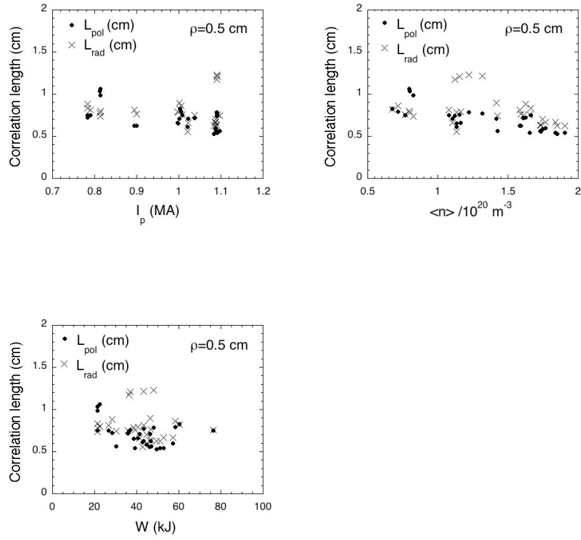
Fig. 4 – Radial and poloidal correlation lengths for the 30 shots in this database, all evaluated at \rho=0.5 cm outside the separatrix. There are only small variations in correlation length over the range of plasma current I_p , line-averaged density \langle n \rangle , and plasma stored energy W in this database (all with q_{95} \sim 3.4 \pm 0.4 ).
