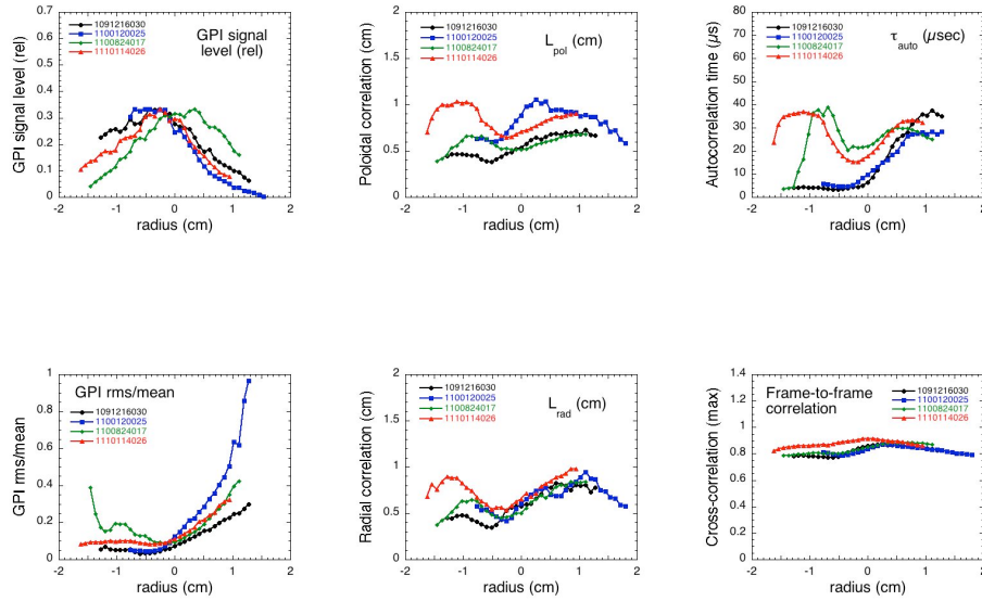
Fig. 5 – Typical radial profiles of turbulence characteristics for four typical shots in this database, averaged over the poloidal analysis region shown in Fig. 2. At the top left are the relative GPI signal profiles, at the bottom left are the relative GPI fluctuation levels, in the middle are the poloidal and radial correlation lengths, at the top right are the autocorrelation times, and at the bottom right are the maximum cross-correlation coefficients from the frame-to-frame velocity analysis.
