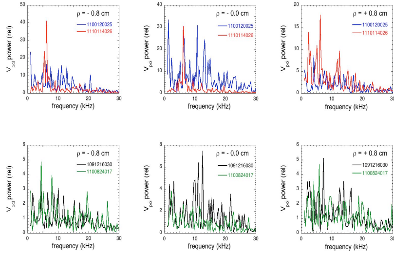
Fig. 10 – Frequency spectra of V_{pol} for the four typical shots of Fig. 6, for three different radii \rho = -0.8 cm, 0.0 cm, and +0.8 cm. These are power spectra averaged over 20 msec for each case. Note the varying vertical scales for each plot.
