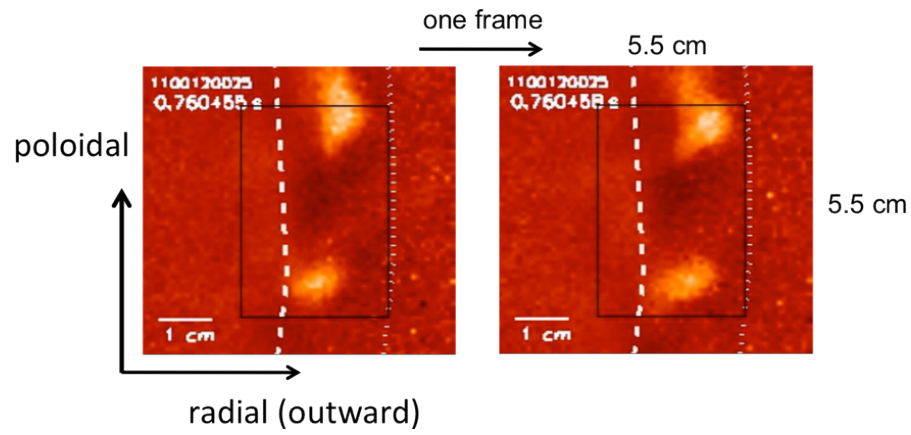
Fig. 2 – Example of two pair of successive normalized images separated by 2.5 \mu s , each with an exposure time of 2.2 \mu s . The signal level is shown in a false color scale, the separatrix is the dashed white line, the limiter (RF antenna) shadow is shown by the dotted white line, and the black box is the data analysis region.
