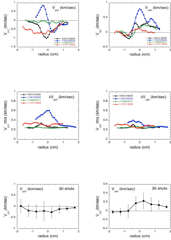
Fig. 6 - Radial profiles of the poloidally-averaged V_{pol} and V_{rad} for four typical shots (top), the RMS fluctuation levels in these velocities (middle), and average of these velocities for the 30 shot database (bottom). There is a fairly wide range of profile shapes for V_{pol} within this radial range, but on average the poloidal velocity is \sim 0.2 km/sec in the ion diamagnetic direction in the SOL. There but is a fairly consistent outward V_{rad} in the SOL of \sim 0.2 km/sec, but a slight reversal to an inward V_{rad} inside the separatrix.
