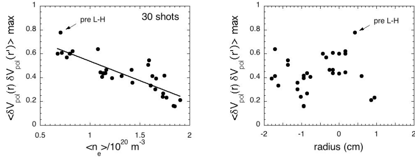
Fig. 12 – At the left is the maximum of the normalized cross-correlation coefficient \langle \delta V_{\text{pol}}(r-\Delta/2) \delta V_{\text{pol}}(r+\Delta/2) \rangle , where \Delta=0.35 cm, for all shots in Table 1. This correlation increases with decreased line-averaged density, and is largest for the 'pre-L-H' shot with a subsequent L-H transition (1110114032). The radius of this maximum cross-correlation coefficient is shown at the right.
